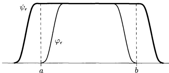
Figure 3. The functions \varphi_\epsilon and \psi_\epsilon in Lemma 2.15
